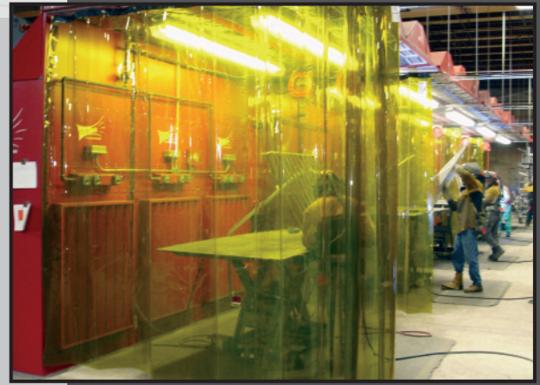
Multiple Clean Air Booths with Regain Air in Welding/Grinding Operation
